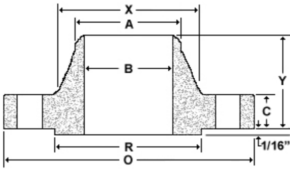
Weld Neck
