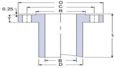
LONG WELD NECK "LWN"
