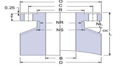
EQUAL BARREL "E"
