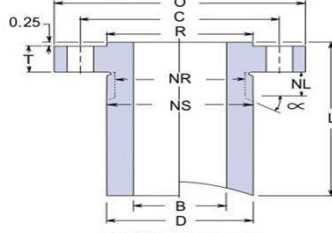
HEAVY BARREL "HB"
